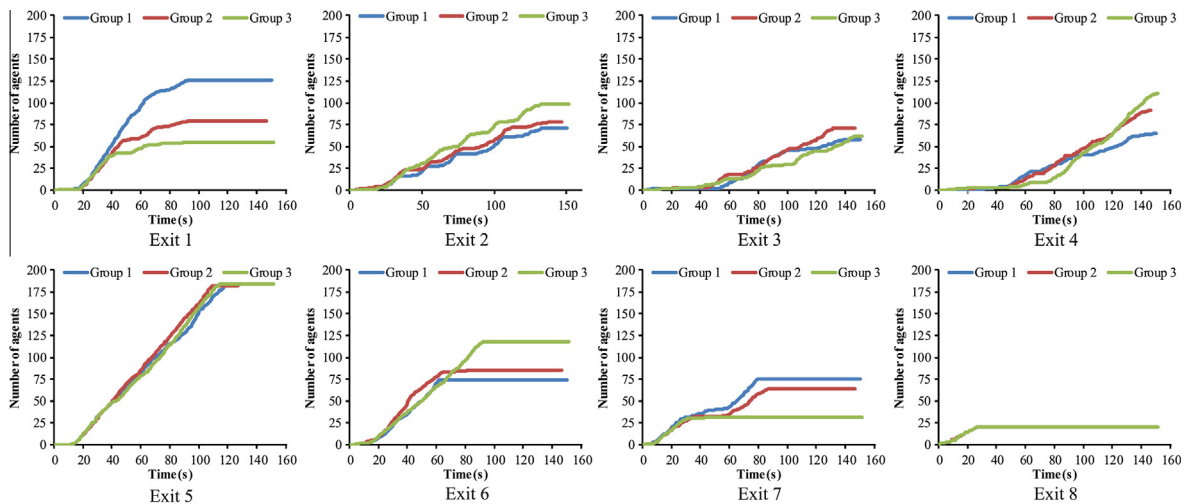
Fig. 11. The cumulative agents passing through each exit during Scenario Three for each group of evacuees.
