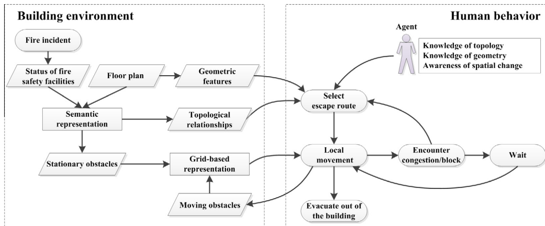
Fig. 1. The framework of agent-based building evacuation simulation combining human behavior with predictable spatial accessibility.
