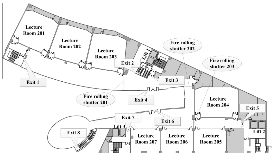
Fig. 6. The floor plan of the second floor of a campus building.
