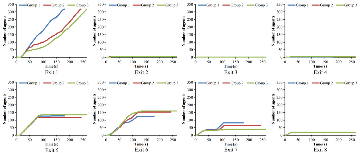
Fig. 10. The cumulative agents passing through each exit during Scenario Two for each group of evacuees.
