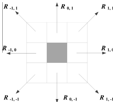
Fig. 3. The repulsion force that is caused by the obstacles in the surrounding cells.
