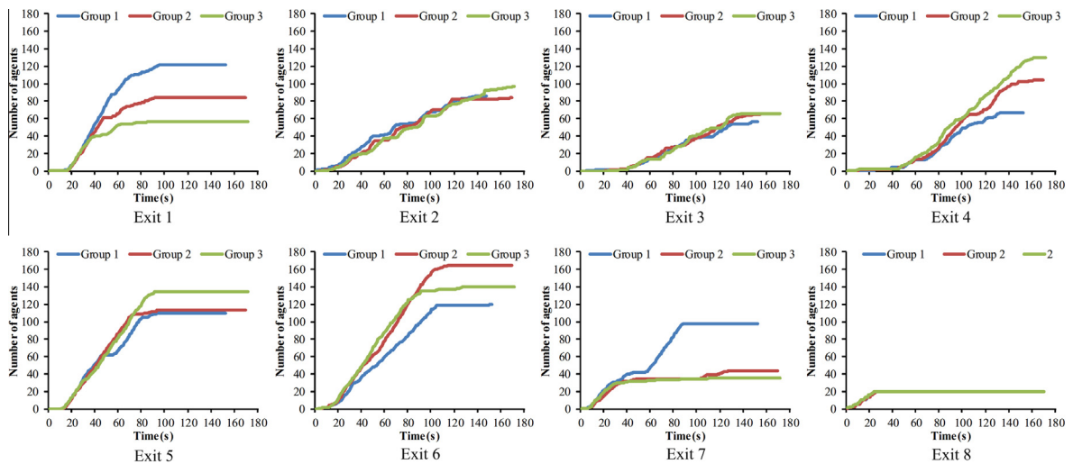
Fig. 9. The cumulative agents passing through each exit during Scenario One for each group of evacuees.
