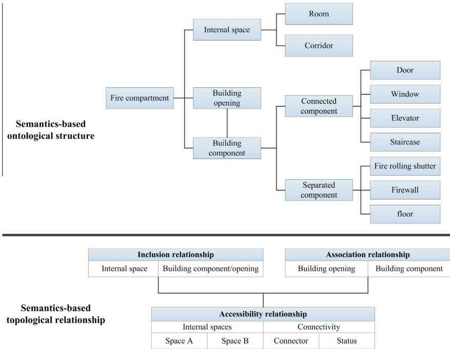
Fig. 2. The semantic ontologies for building fire safety and semantics-based topological relationships.
